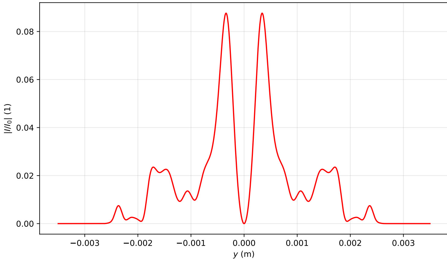
Intensity profile I(x = 0, y, z = 3.742)/I_0 , P_{in}=7.0P_{cr} , artificial time
